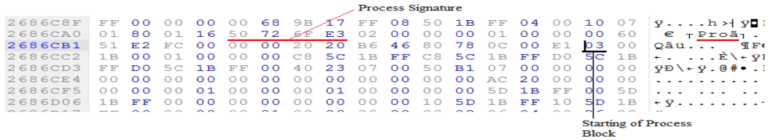
Figure 1. Offset for proã of metasploit.exe block at 0x2686ca4 (Starting of process block at 0x2686cc0)
