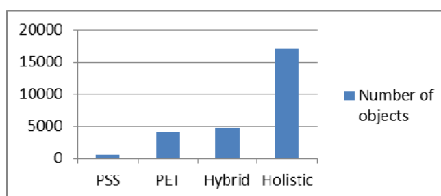
Figure 2. Number of retrievable objects from DFRWS memory dump
